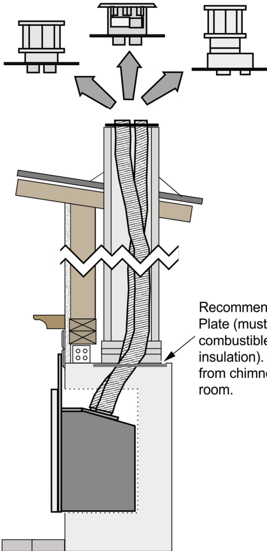
Factory Built (Metal) Wood-Burning Fireplace
