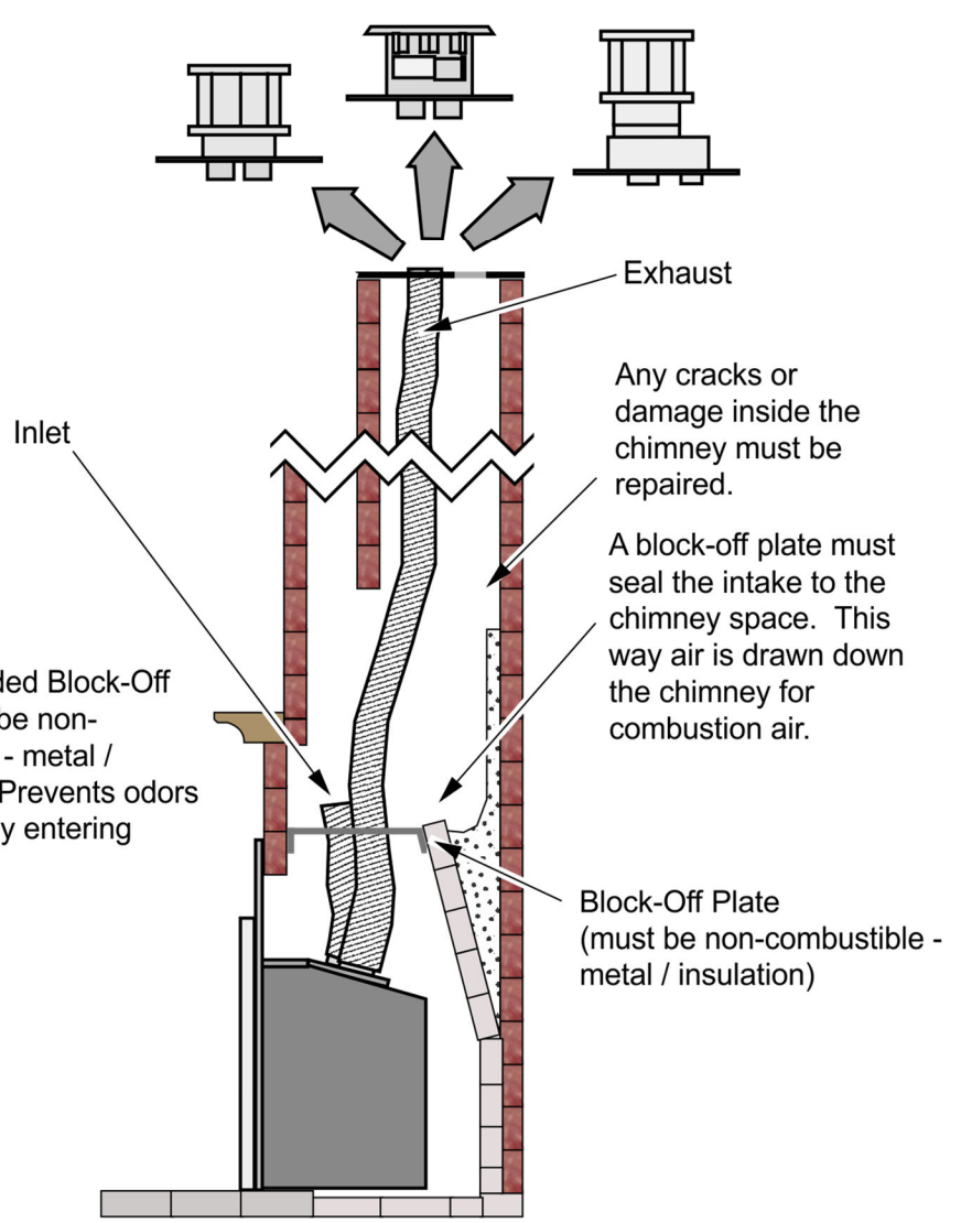
Masonry Fireplace
